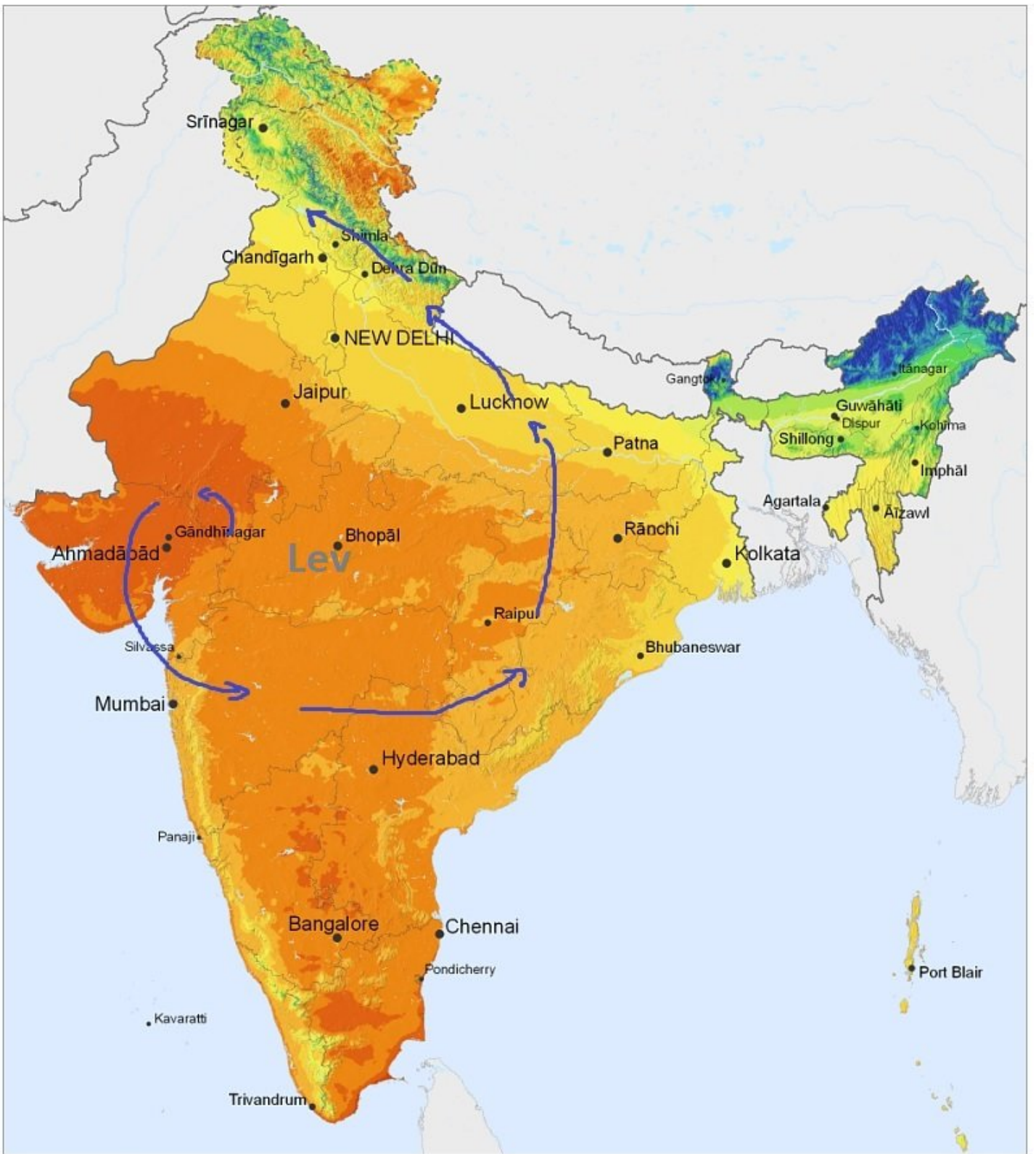
Average annual sum (2005-2010) < 1250 1400 1550 1700 1850 2000 2150 > kWh/m 2
